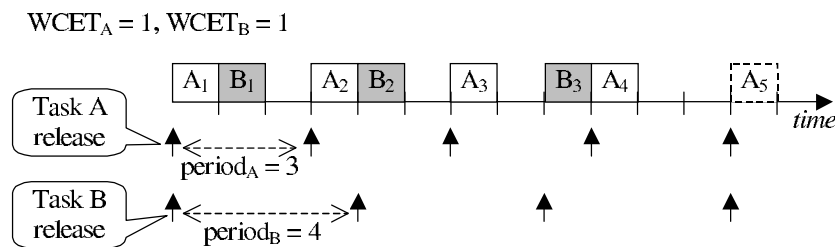
Figure 1. Example showing two periodic hard-real-time tasks.
